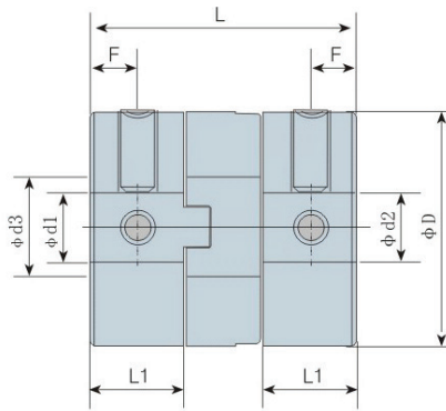
Setscrew Type
