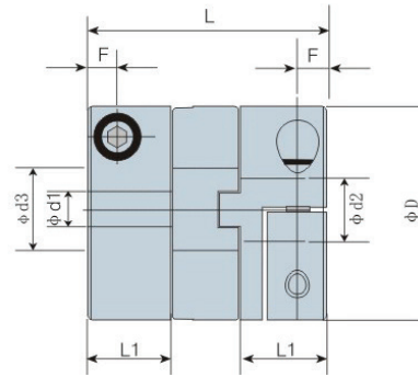
Clamp Type
