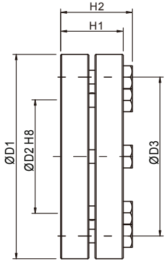
SHRINK DISC POWER LOCK
